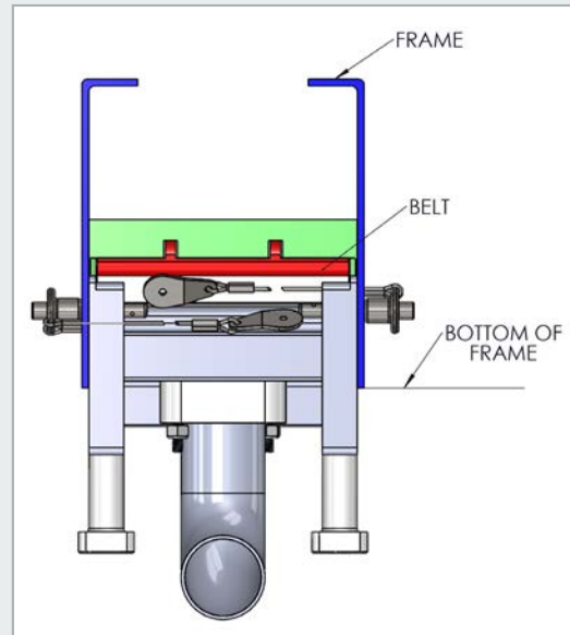
PUREBELT® BOTTLING LINE BELT CLEANING SYSTEM: Belt cleaning system cleans bottling line belts in place automatically with dry steam and vacuum extraction..... Call for Price
